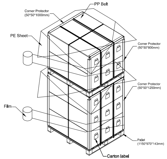
Figure. 7-2 Packing method
